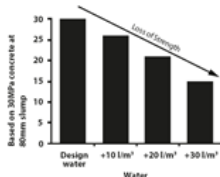
EFFECT OF EXCESS WATER ADDITION ON CONCRETE COMPRESSIVE STRENGTH
